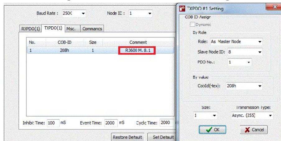
Figure 58: FBs-24MC TXPDO Setting
