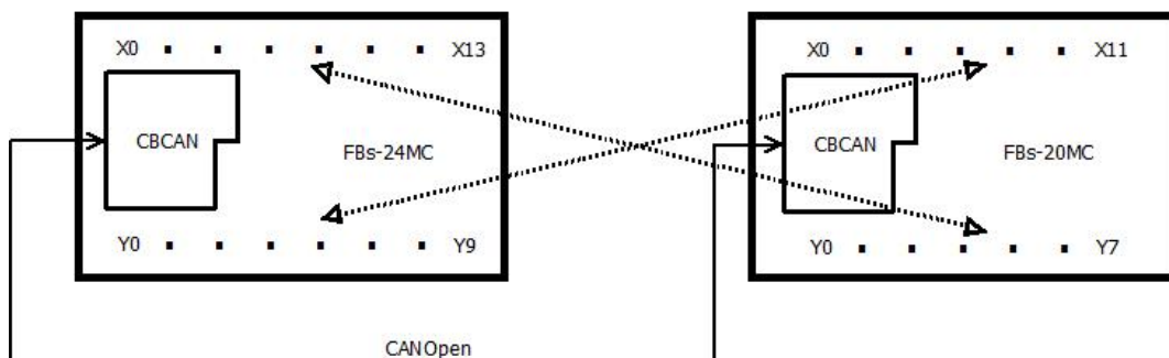
Figure 56: FBS-24MC connect to FBS-20MC
