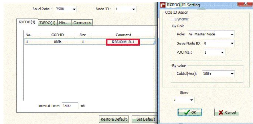
Figure 57: FBs-24MC RXPDO Setting
