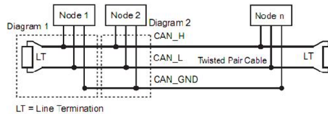
Figure 3: CANopen line termination
