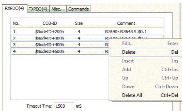
Figure 49: Removing RXPDOs
