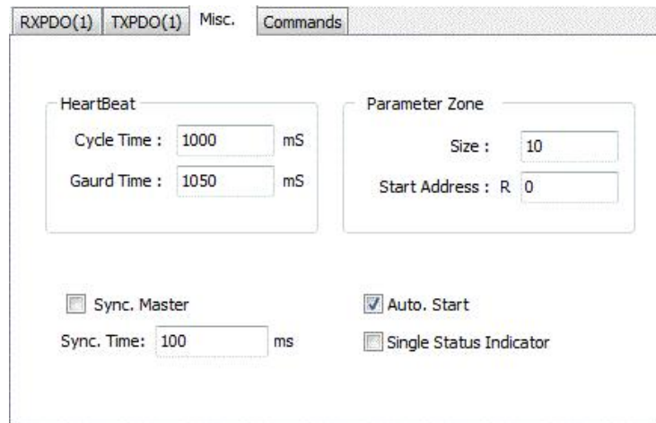
Figure 59: FBS-24MC Misc Setting
