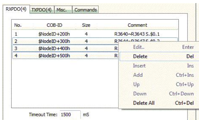
Figure 37: Removing RXPDOs
