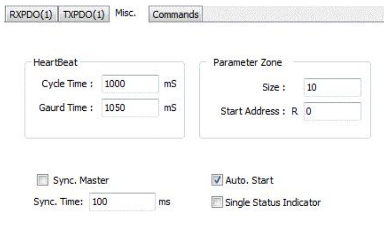
Figure 62: FBs-20MC Misc. Setting
