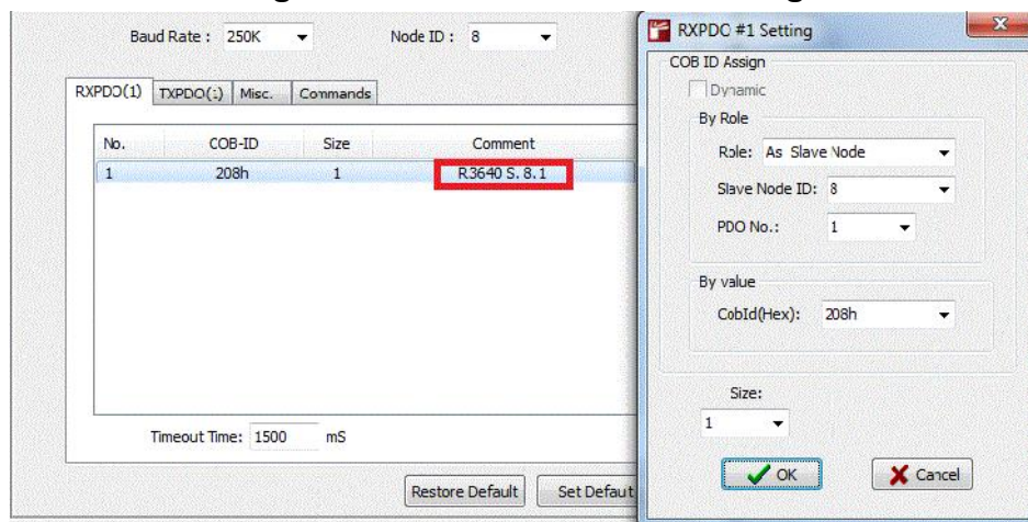
Figure 60: FBS-20MC RXPDO Setting
