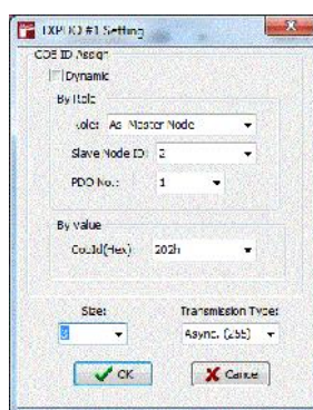
Figure 53: TxPDO settings
