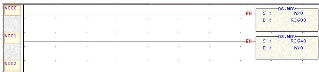
Figure 63: FBs-24MC and FBs-20MC Ladder Program
